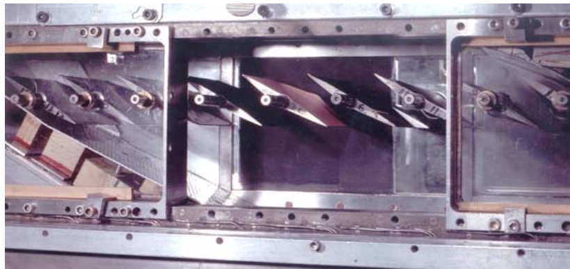
Fig. 1. View of the NASA TFC test section.
