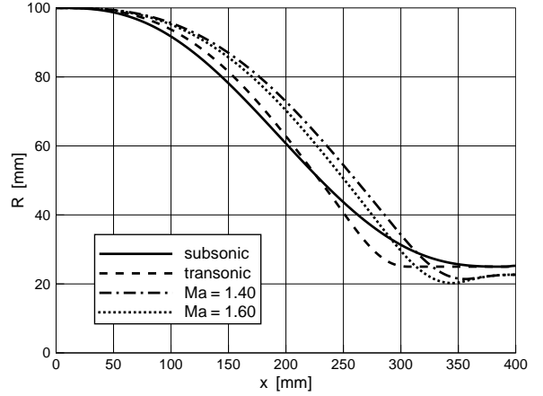
Figure 4: Contours of different nozzles
