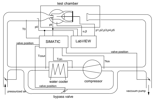
Figure 8: Flow control and data acquisition at SEG (schematic)
