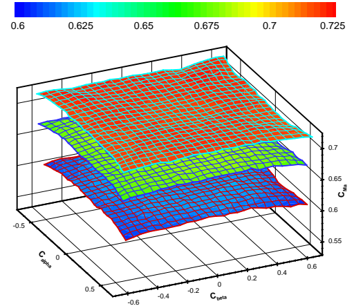
Figure 17: Measured coefficients at Ma = 0.7, 0.8, 0.9
