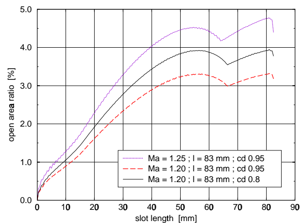
Figure 6: Open area ratio of slotted nozzle (total slot width to nozzle perimeter) for different design Mach numbers and discharge coefficients
