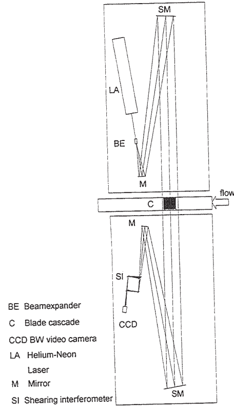
Fig.6 Setup for heterodyne differential interferometry
