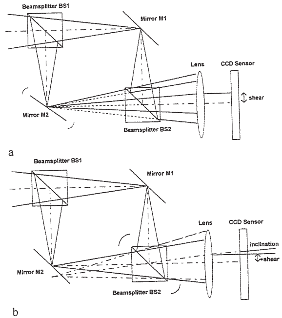
Fig.7 Shearing interferometer for heterodyne differential interferometry a) adjustment of shear b) adjustment of inclination (Carrier fringe system)
