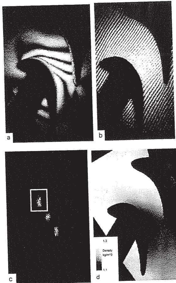
Fig. a) Holographic interferogram of subsonic flow without and b) same interferogram with carrier fringe system heterodyned c) frequency spectrum of b) with window for filter process d) resultant density map
