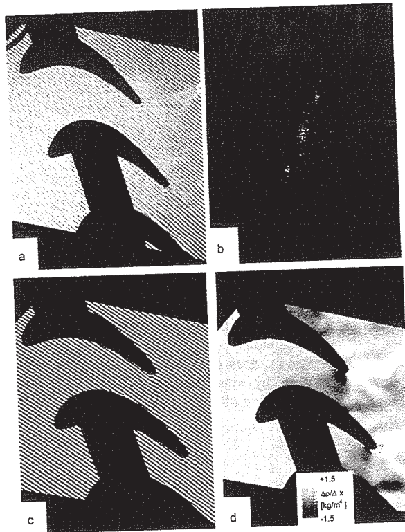
Fig.9 a) Heterodyne differential interferogram, b) frequency spectrum, c) modulo 2\pi phase map, d) density gradient map
