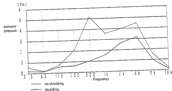
Fig.10 Sound pressure on an optical element caused by the continuously running cascade with and without shielding of the optical setup.
