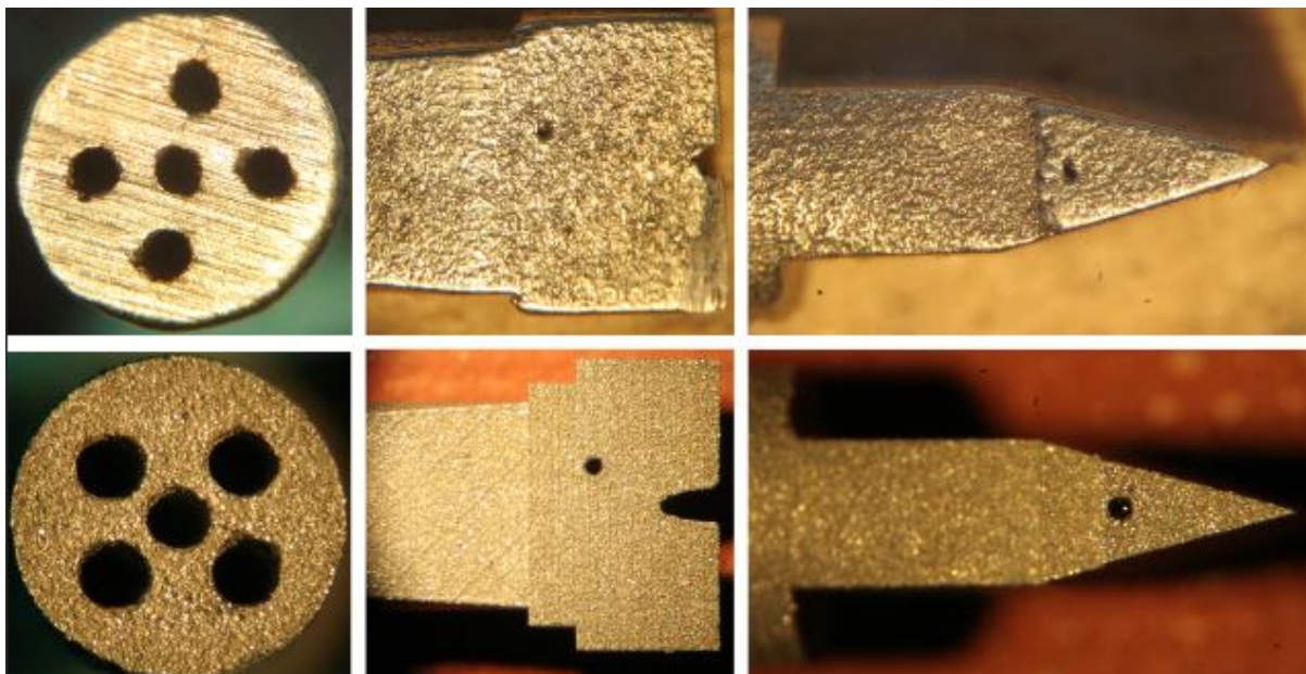
Figure 5: Raw sintered probe head build with a layer thickness of 10 \dots 50\text{ }\mu\text{m} (upper row) and with 1 \dots 5\text{ }\mu\text{m} (bottom row)
