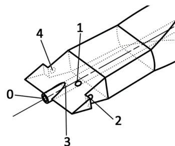
Figure 6: Positions and labeling of the pressure taps at the MWP head
