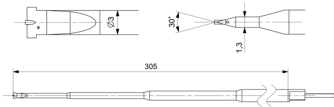
Figure 7: Dimensions of Miniaturized Wedge Probe (MWP) with probe shaft
