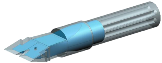
Figure 4. Design of the sintered raw probe head with additional material (grey) to the final MWP head (blue)
