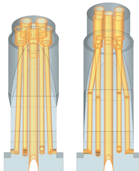
Figure 3: Internal pressure duct design for EDD (left) and AM (right) method
