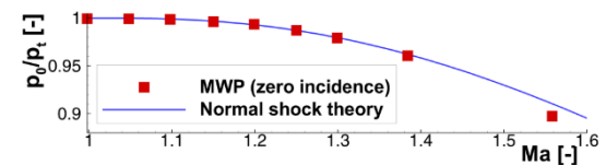
Figure 9: Total pressure measurement in supersonic flow at zero incidence compared to normal shock theory
